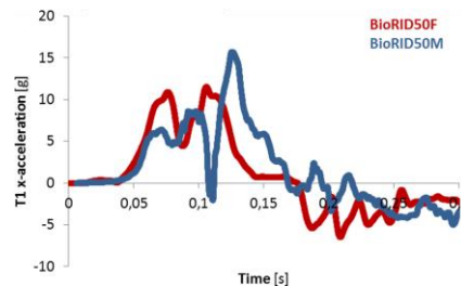
Figure 2: Example of T1 x-acceleration of the two dummy sizes in the same seat (Fig. 1). The female size dummy, BioRID 50F, shows a higher acceleration magnitude during the initial 0–75 ms phase. This is the time window when the neck undergoes the characteristic whiplash s-shape motion and where pressure transients peak in the spinal canal.
