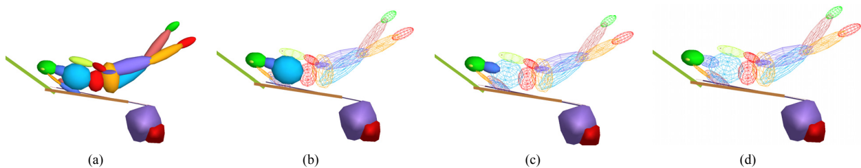
Figure 2. An illustrative example of the four head boundary conditions or configurations for multi-body pedestrian model at 5 ms before head impact: (a) body conf., (b) thorax conf., (c) neck conf., (d) head conf
