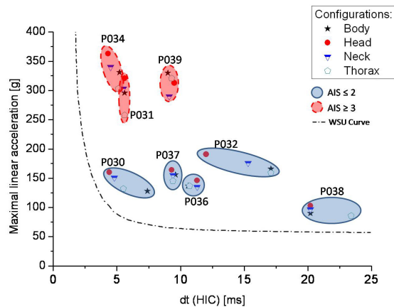
Figure 8. Maximum linear acceleration at the centre of gravity of the head function of impact time duration by case for the four configurations
