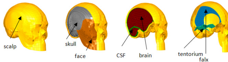
Figure 4. Strasbourg University Finite Element Head Model (SUFEHM) components
