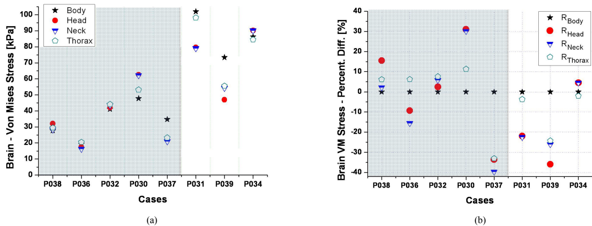
Figure 10. (a) Brain maximum Von Mises stress by case and by configuration and (b) percentage difference between configurations value for brain Von Mises stress by case, classified by increasing AIS. In grey background, cases with AIS ≤ 2, in white background cases with AIS ≥ 3
