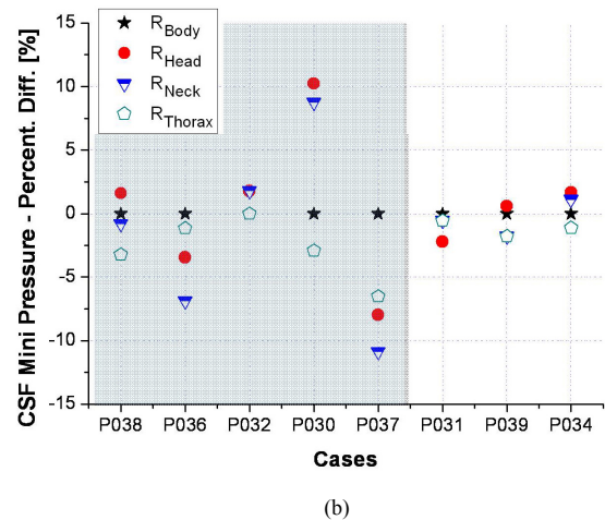
Figure 9. (a) CSF minimum pressure by case and by configuration and (b) percentage difference between configurations value for CSF minimum pressure by case, classified by increasing AIS. In grey background, cases with AIS≤2, in white background cases with AIS≥3
